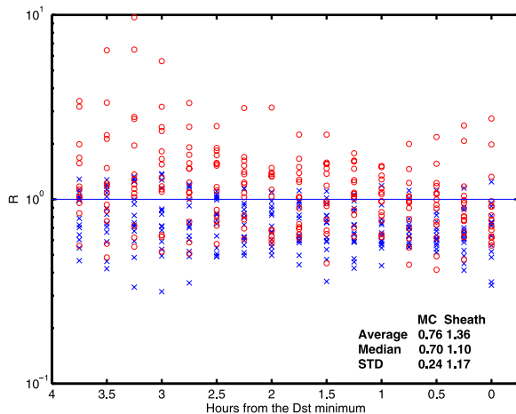
Figure 3. |ASYH|/|SYMh| during 14 sheath (red circles) and 14 magnetic cloud (blue crosses) driven storms (plotted logarithmically). Average, median and standard deviation (STD) for magnetic cloud (MC) and sheath data sets are given in the lower right hand corner.
