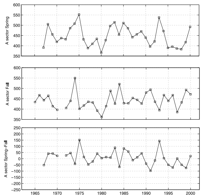
Figure 5. SW speeds (in km/s) in the away sector; top: 3-month averages in Spring; middle: 3-month averages in Fall; bottom: Spring-Fall difference.
