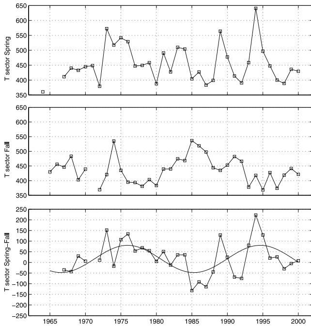
Figure 4. SW speeds (in km/s) in the toward sector; top: 3-month averages in Spring; middle: 3-month averages in Fall; bottom: Spring-Fall difference. The curve is the best fitting sinusoid.
