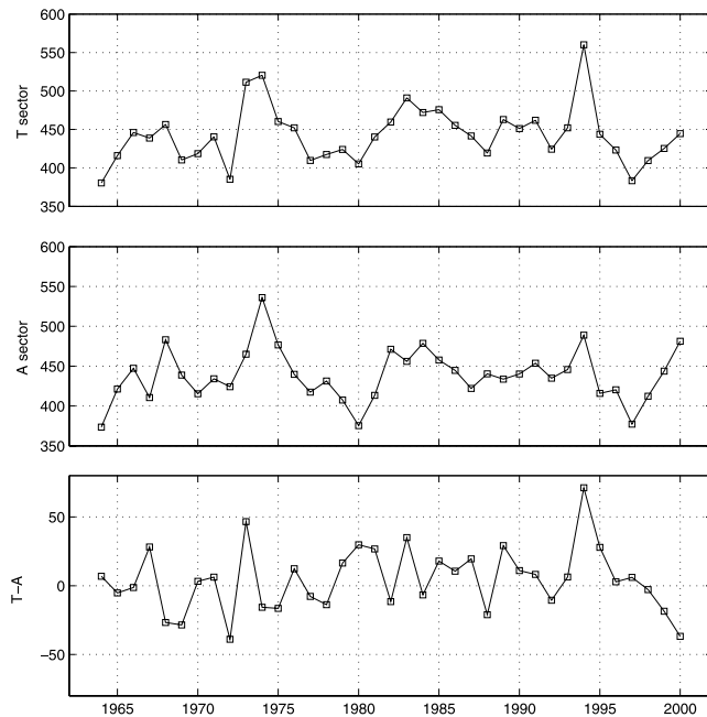
Figure 3. Annual SW speeds (in km/s); top: in the toward sector; middle: in the away sector; bottom: toward-away sector difference.
