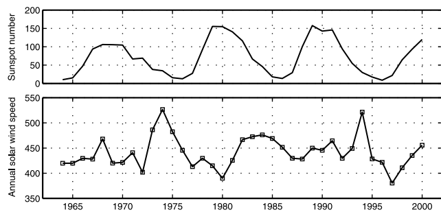
Figure 1. Top: annually averaged sunspot numbers for 1964–2000; bottom: annually averaged solar wind speeds (in km/s) for 1964–2000.
