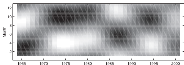
Figure 2. Filtered annual variation of SW speed in intensity coding, white (black) representing high (low) speeds. Vertical scale presents the variation in one year from January to December.
