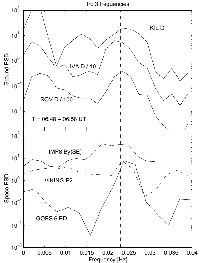
Figure 3. Selected power spectra from the ground (upper panel) and space (lower panel). The vertical dashed line corresponds to 23 mHz (43 s).
