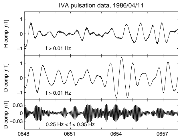
Figure 2. Search-coil magnetometer data from the IVA station during the Viking Pc 1 event. The two upper panels show the Pc 3 waves in the two components (DC trend has been removed); the bottom panel shows the the ground Pc 1 waves in the frequency range of the first Viking Pc 1 region.
