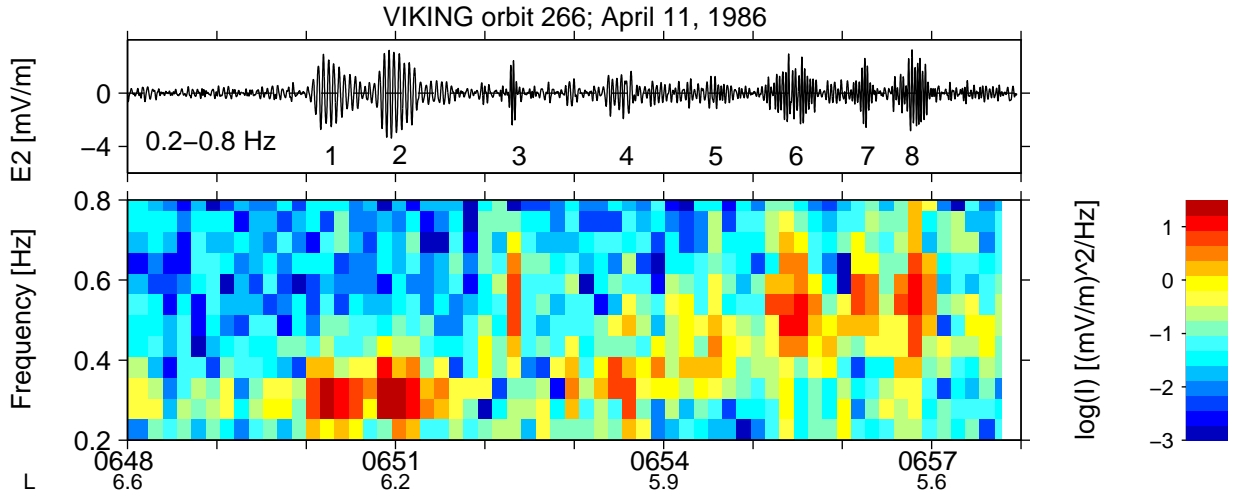
Figure 1. The EMIC wave bursts observed by Viking in the perpendicular electric field component. The two separate wave source regions are seen from the difference in wave frequency at higher (left-hand side) and lower latitudes (right-hand side).
