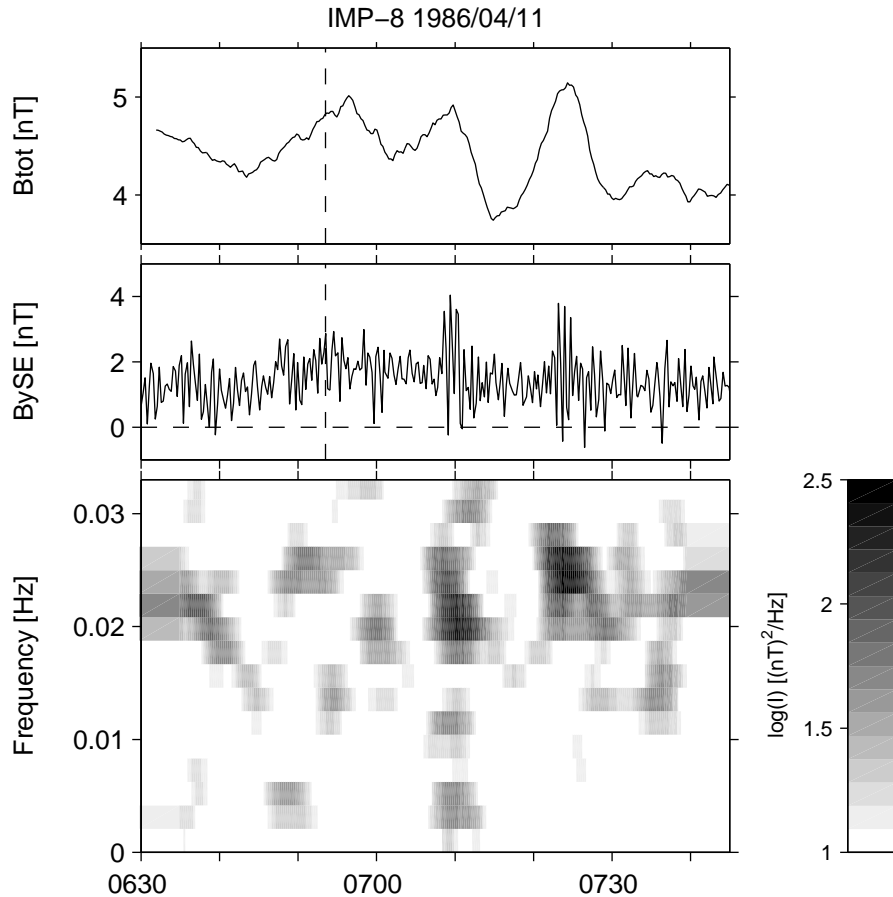
Figure 4. IMF strength (floating average over 5 min) and higher resolution waveform and spectrogram of the upstream wave activity around the Viking event (0650 - 0657 UT; midpoint is indicated by the dashed vertical lines).
